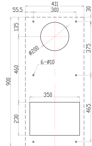
Mounting cut out Drawing as seen from the exterior of the enclosure.
