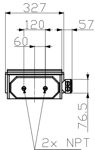
Terminal box - Front view
