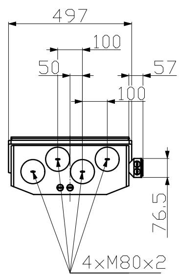
Terminal box - Front view
