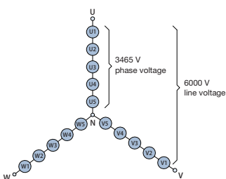
Fig. 3 6 kV configuration
