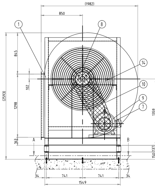
FAN DRIVE SIDE VIEW
