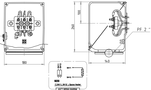
MOTOR TERMINAL BOX ASS'Y
