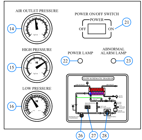
GAUGE PANEL DETAIL
